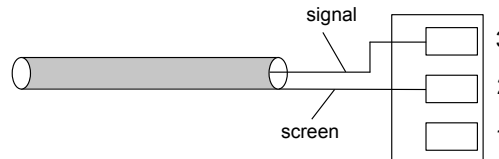
Connecting an unbalanced source
