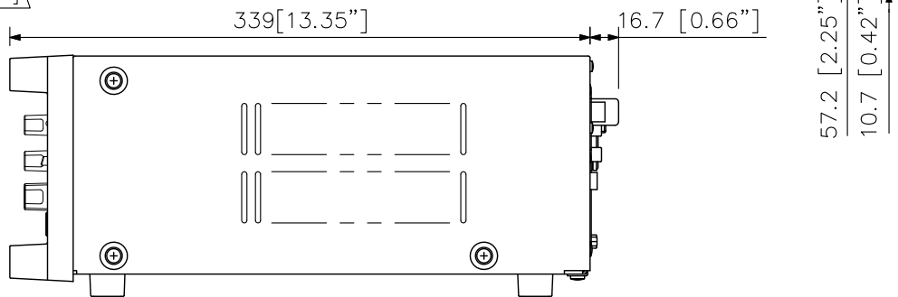
Side View
