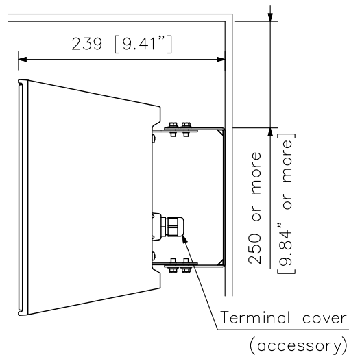
Vertical installation
