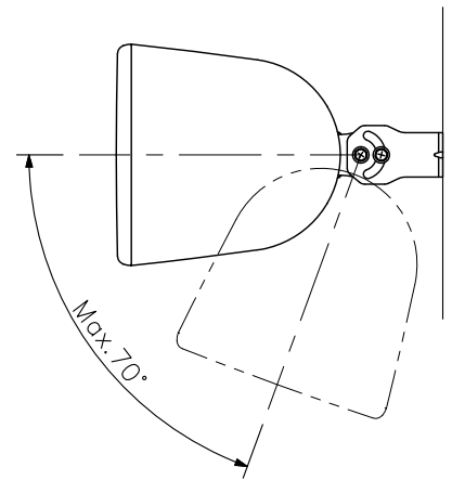
Horizontal installation
