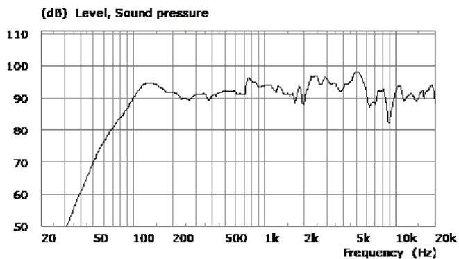
Frequency Response
