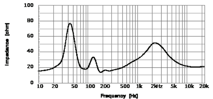
Phase/Impedance Response
