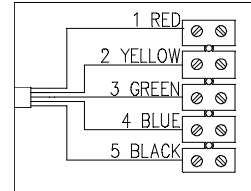
CONNECTION DIAGRAM
