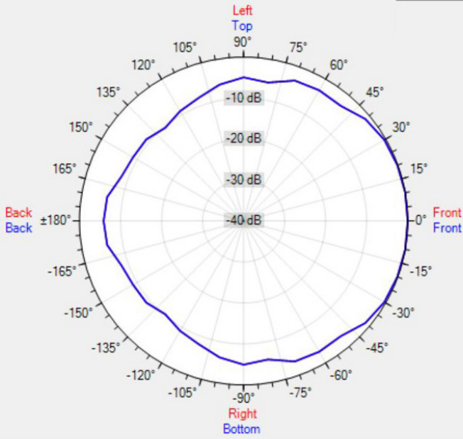
Data Shown: MP26 (Apart Audio) Display Parameters: Frequency: 1000Hz (1/24th Octave)
