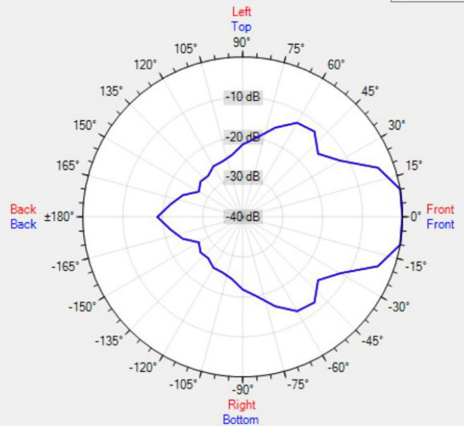
Data Shown: MP26 (Apart Audio) Display Parameters: Frequency: 8000Hz (1/24th Octave)
