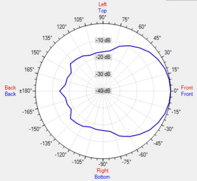
Data Shown: MP26 (Apart Audio) Display Parameters: Frequency: 2000Hz (1/24th Octave)
