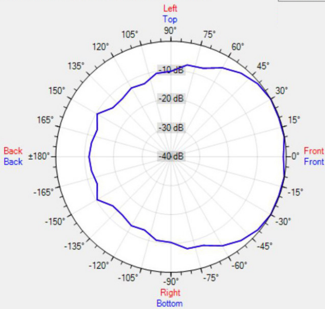
Data Shown: MP26 (Apart Audio) Display Parameters: Frequency: 4000Hz (1/24th Octave)
